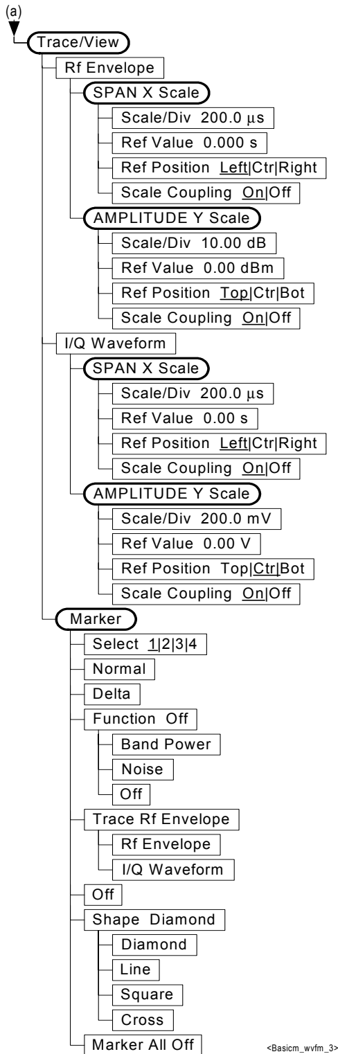
Figure 6-9 Waveform (Time Domain) Measurement Key Flow (3 of 3)
