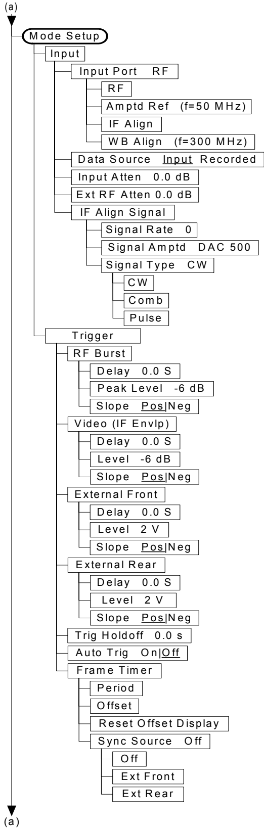
Figure 6-11 Power Stat CCDF Measurement Key Flow (2 of 3)
