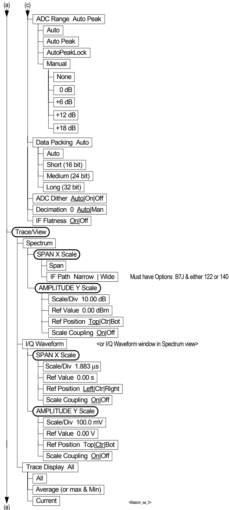
Figure 6-5 Spectrum (Freq Domain) Measurement Key Flow (3 of 4)
