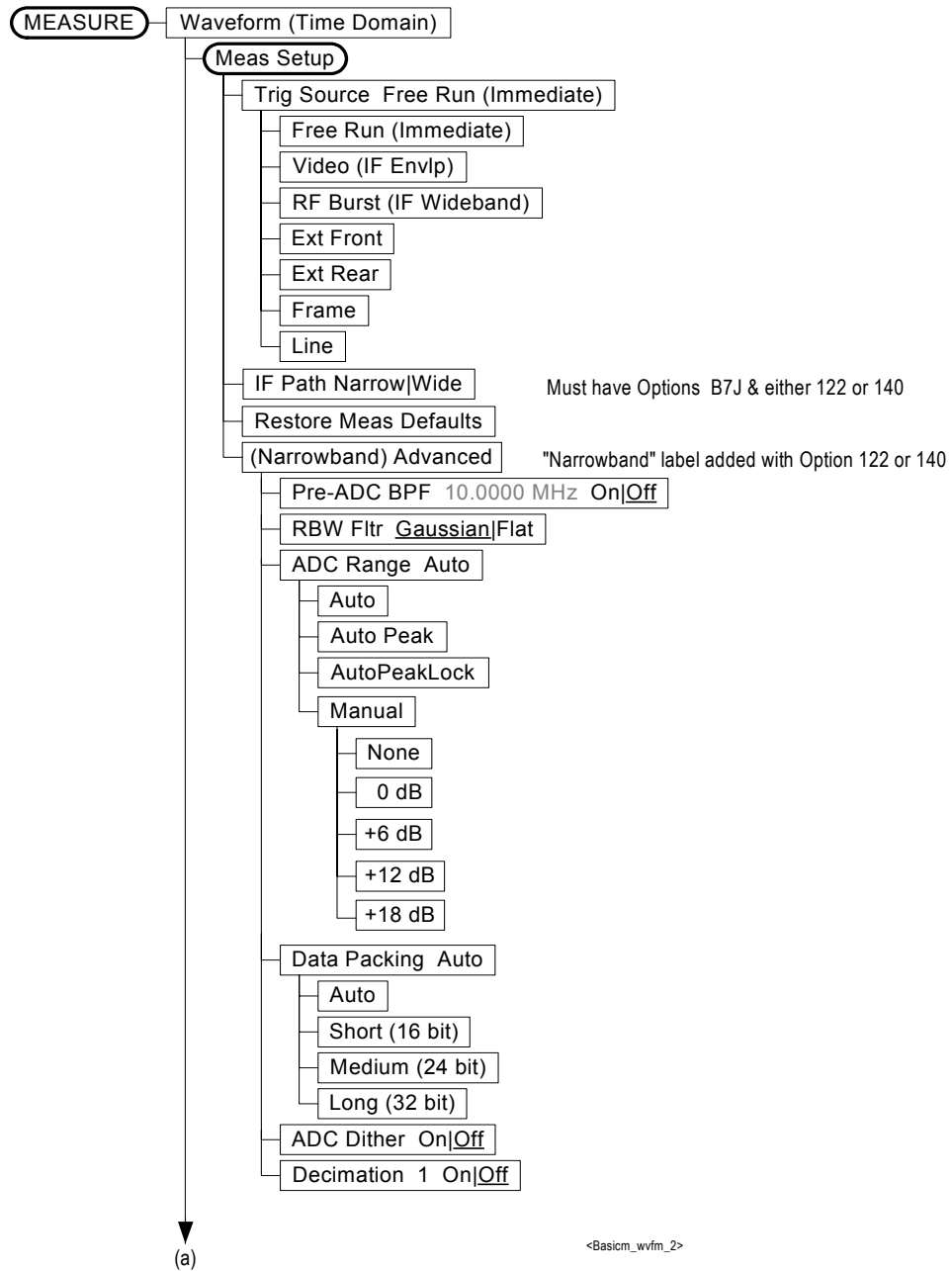
Figure 6-8 Waveform (Time Domain) Measurement Key Flow (2 of 3)
