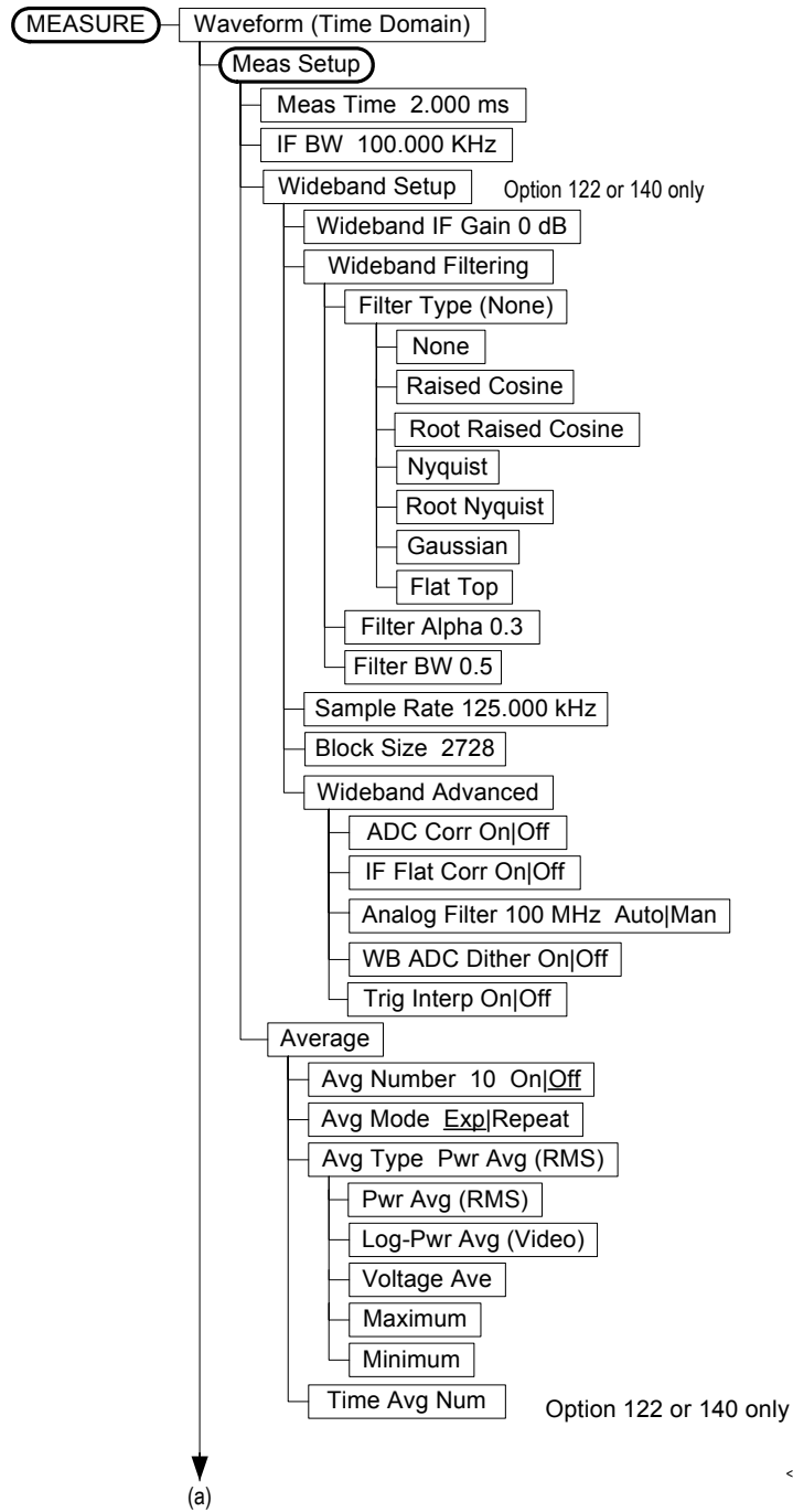
Figure 6-7 Waveform (Time Domain) Measurement Key Flow (1 of 3)
