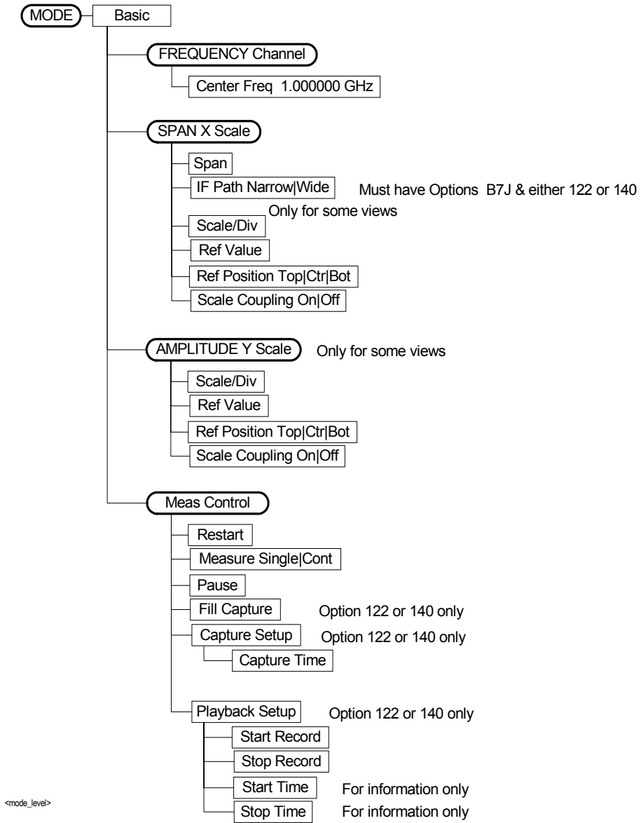
Figure 6-2 FREQUENCY, SPAN, AMPLITUDE & Meas Control Flows
